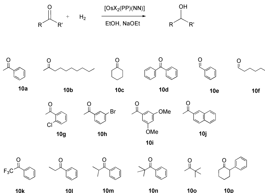
Scheme 3. Hydrogenation of ketones and aldehydes 10 with the trans and cis Os complexes 3–9 (S/C=10000–200000).
