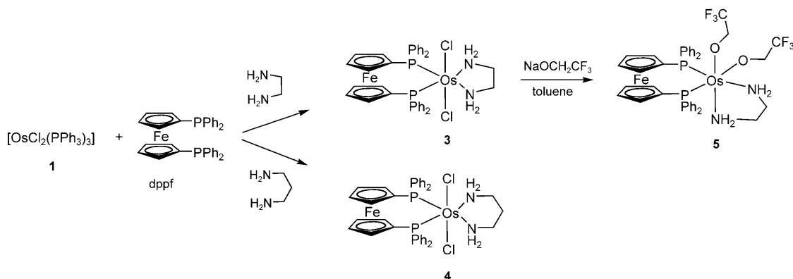
Scheme 1. Synthesis of the complexes [\text{OsX}_2(\text{dppf})(\text{diamine})] (X: Cl, OR).
