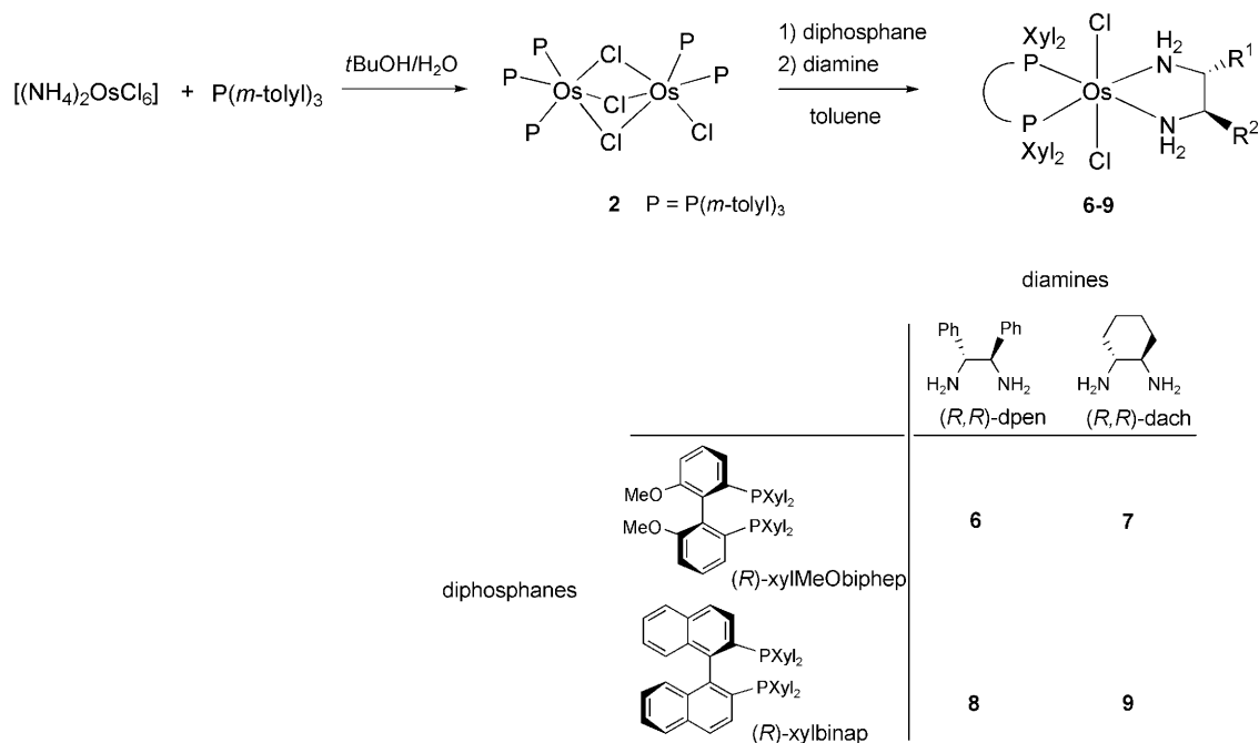
Scheme 2. Synthesis of the novel osmium precursor 2 and the chiral complexes trans - 6–9 .
